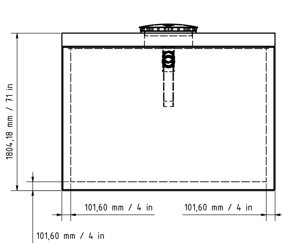
FRONT VIEW
